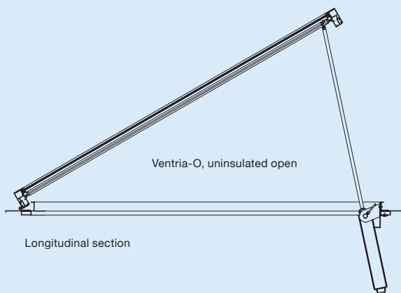
Cross sections
