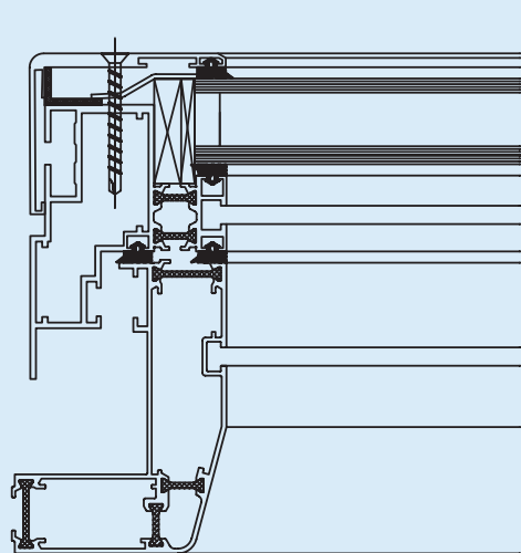
Cold bridge-free
